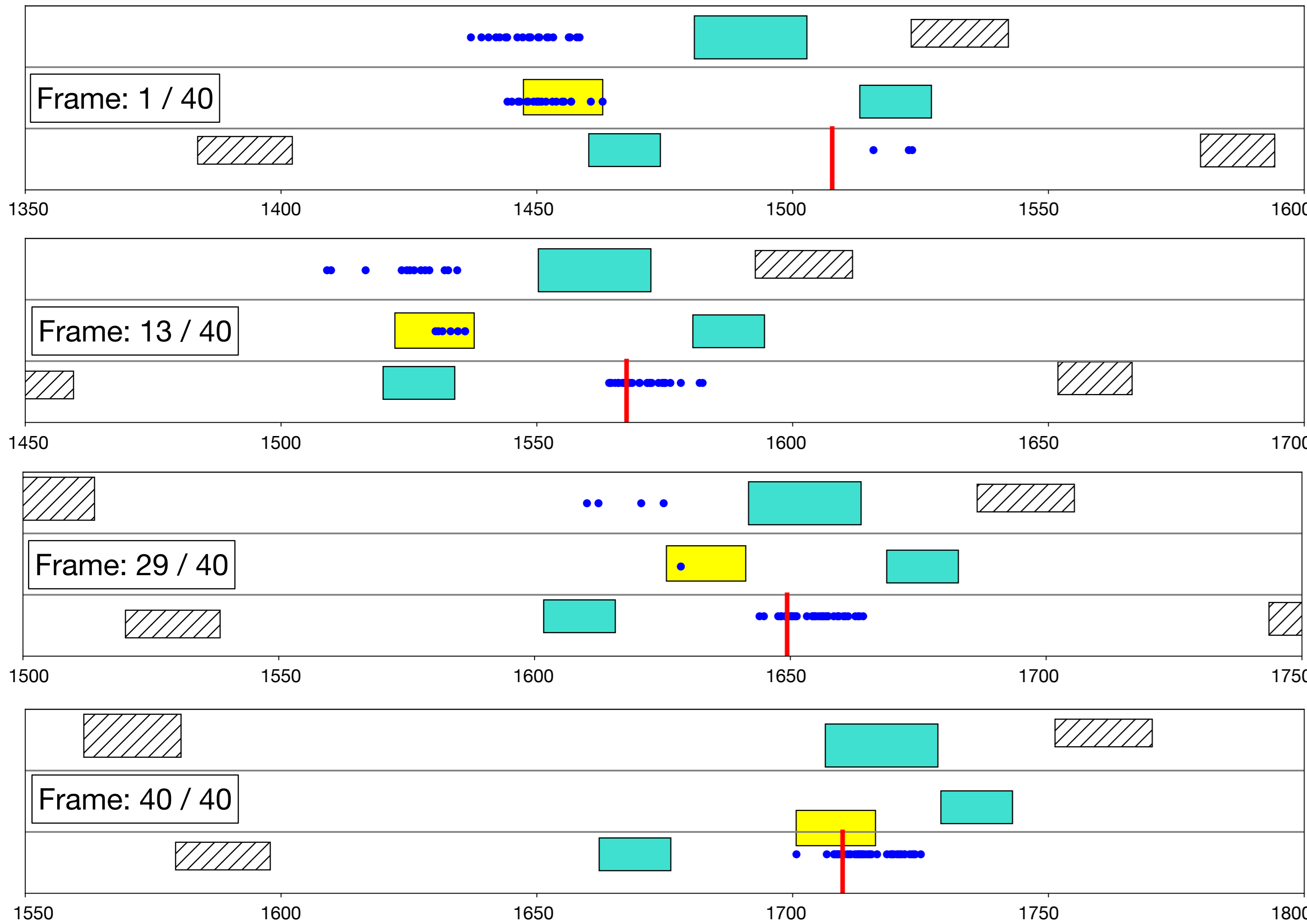
(a) Typical Lane Change
